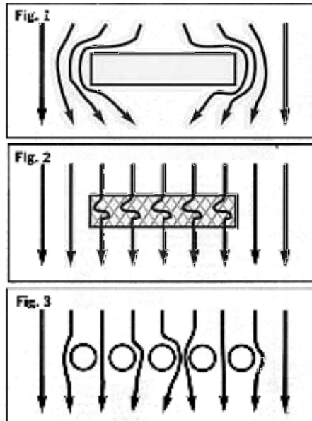
To minimize the degraded shielding effects in discontinuity of induced currents caused, for example, by a required housing vent opening (Fig. 1), proven vent covers such as conductive wire mesh (Fig. 2) can be used, or aperture geometry can be redesigned as in Fig. 3.
